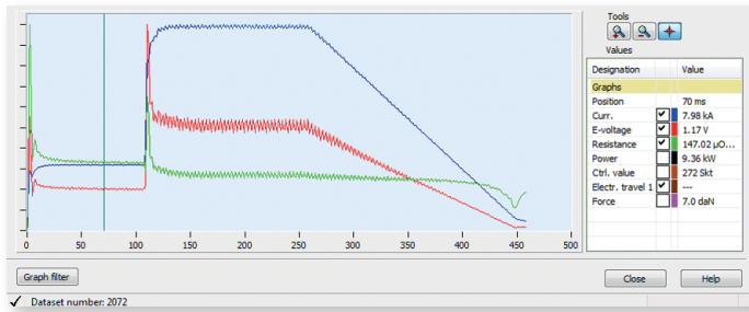
Weld process in X Pegasus HMI
